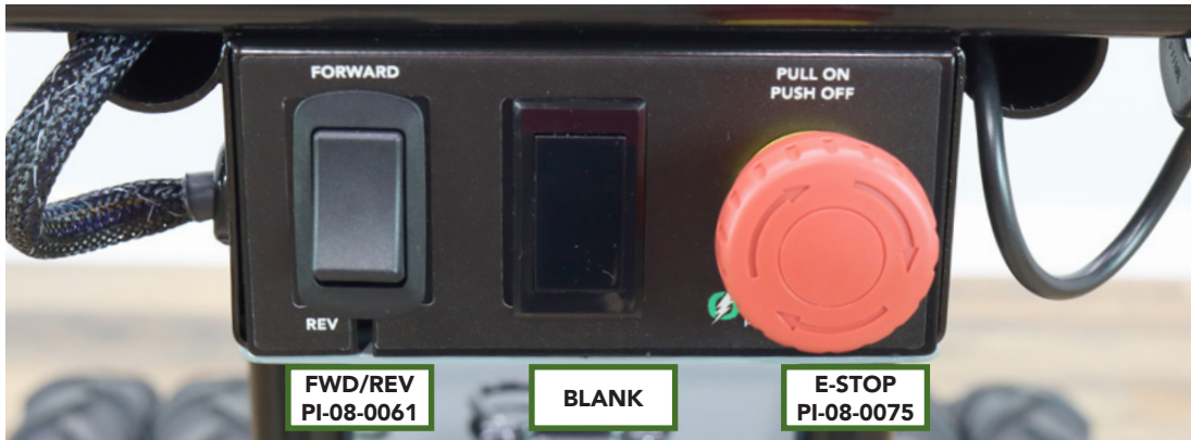
HANDLE CONTROL BOX EXTERIOR
